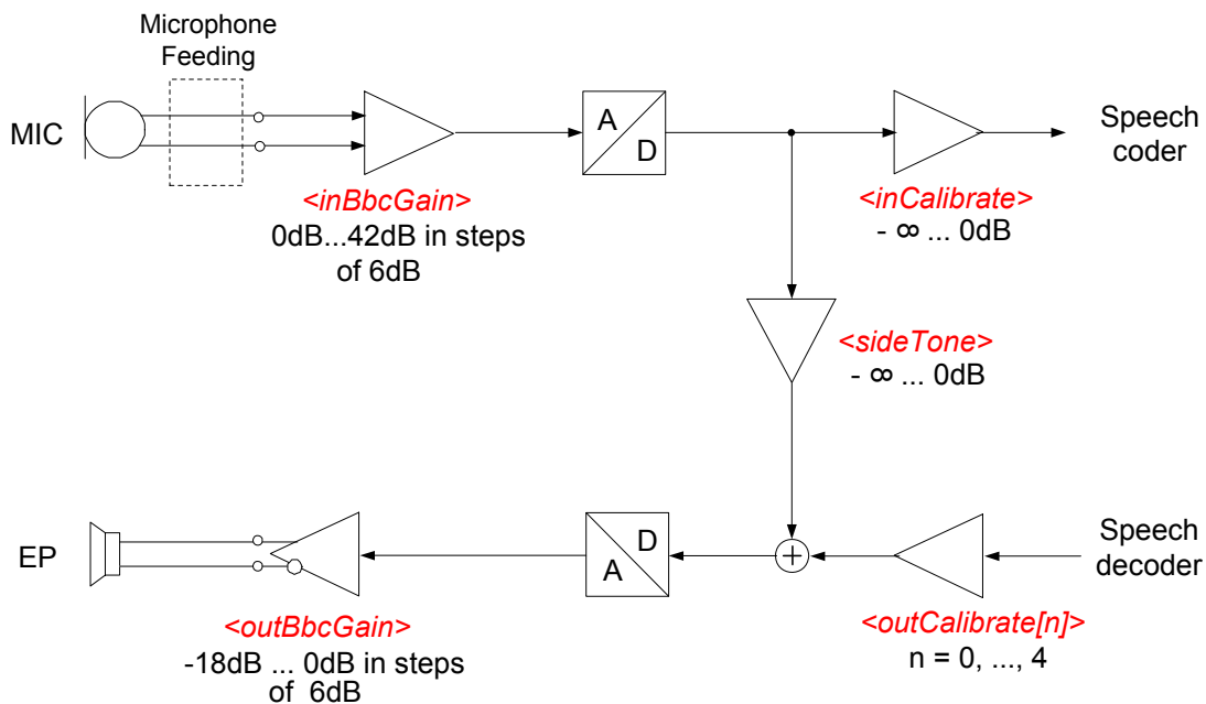
Figure 8: Audio block diagram
