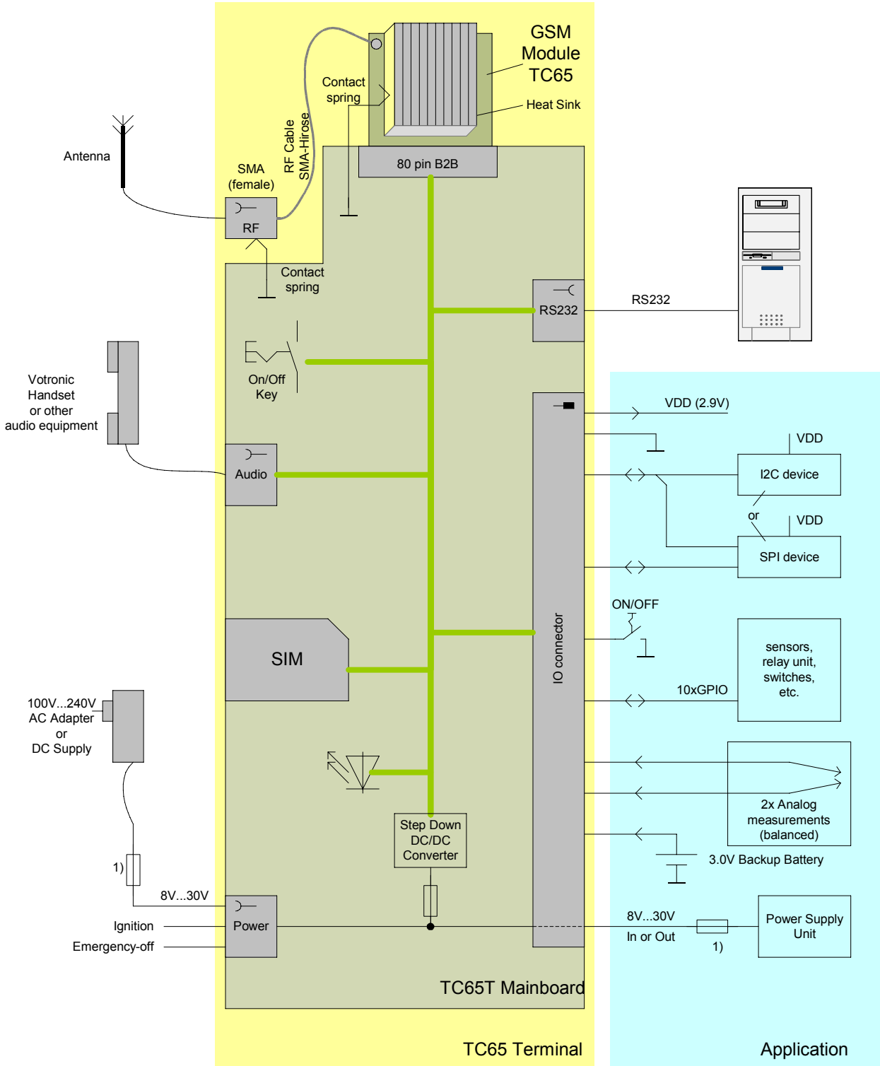
Figure 3: Block diagram
